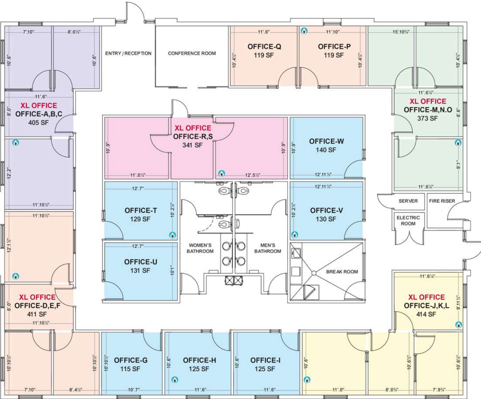
BUILDING-4 FLOOR PLAN TOTAL 4853 SF
