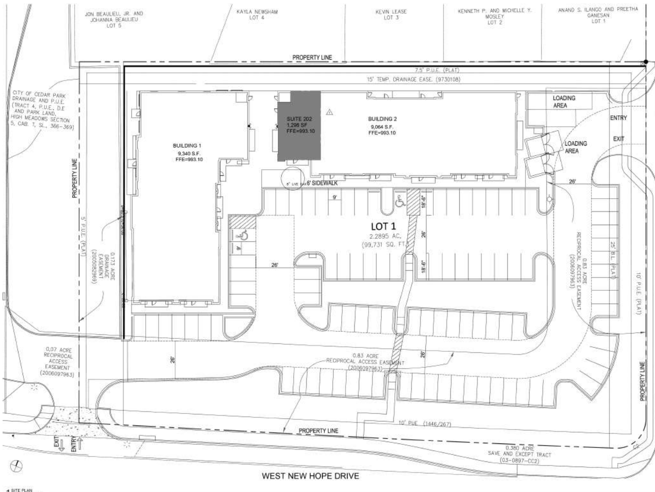
1 SITE PLAN DATE: 03/26/23
